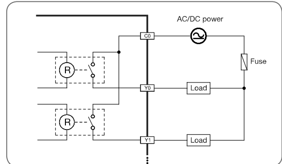
Wiring of relay single-end output
